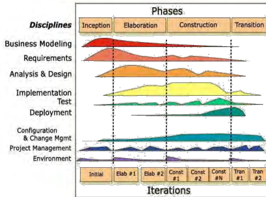
Abbildung 12: Der Rational Unified Process (RUP)[JBR99]
